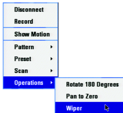
Figure 54. Wiper Submenu
